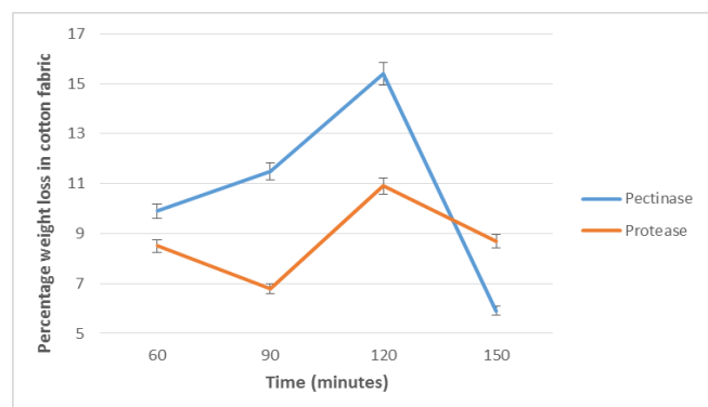
Figure 3 – Effect of different time intervals on the bio-scouring of cotton fabric
