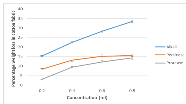
Figure 1 – Effect of different concentrations of alkali, pectinase and protease on cotton fabric
