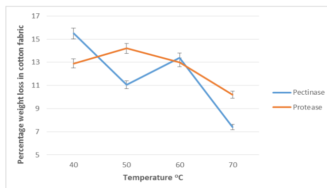
Figure 2 – Effect of different temperatures on bio-scouring of cotton fabric
